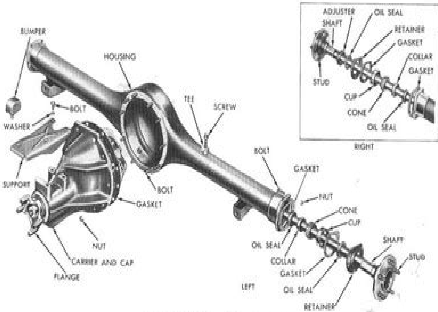
Fig. 1-8-3/4" Rear Axle Assembly
