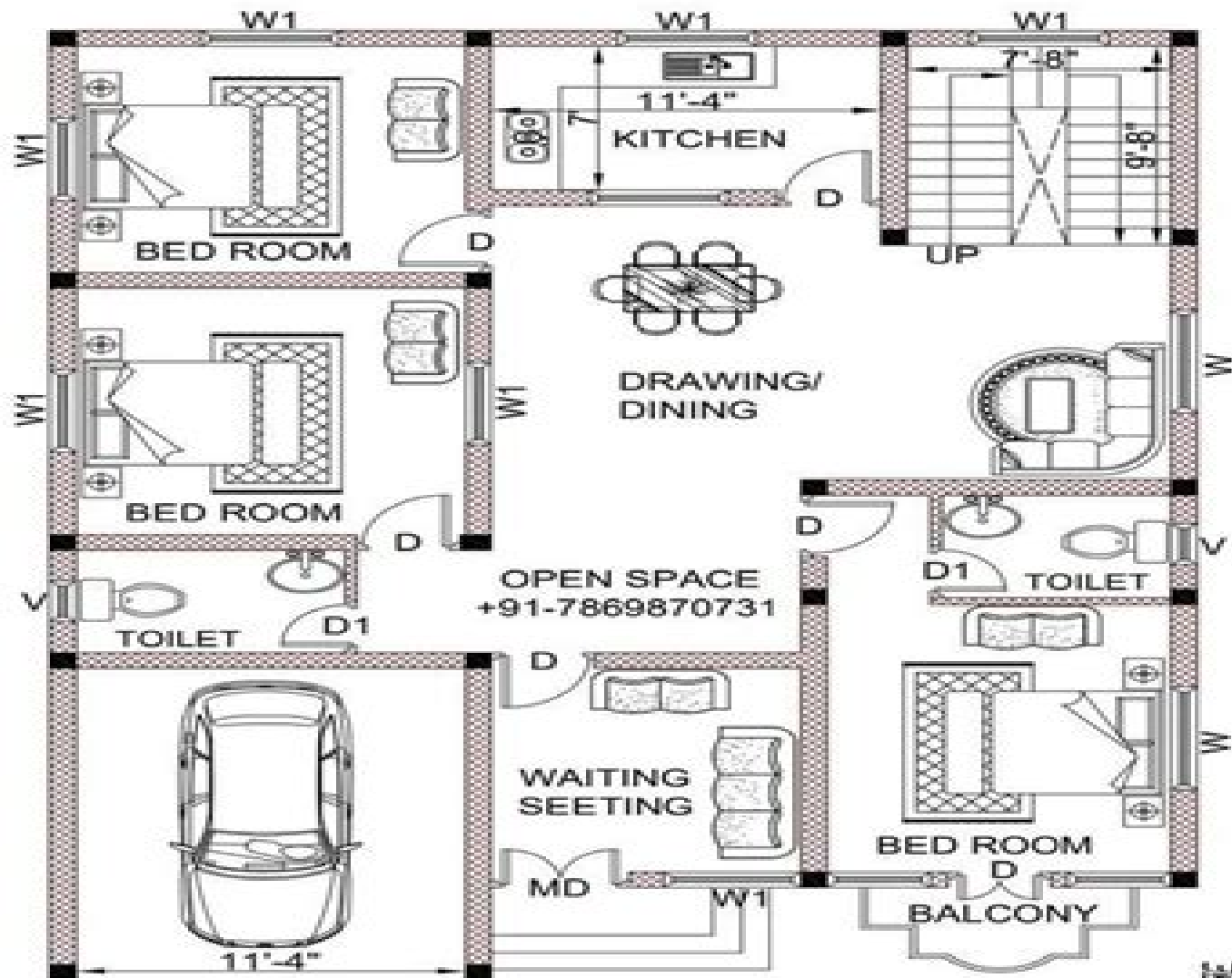
PROPOSED G - FLOOR PLAN (1518 SQFT)
