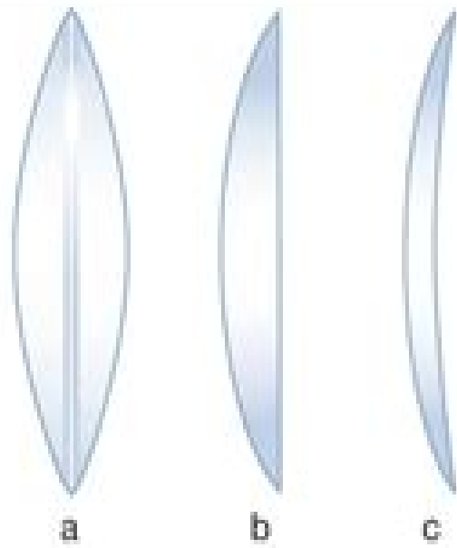
converging lenses
