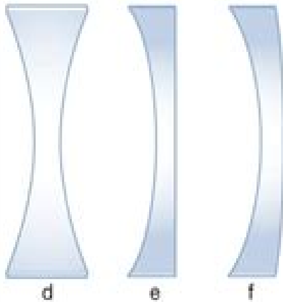
diverging lenses
