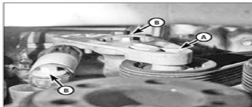
22.7a Insert a ratchet or breaker bar into the square hole (A) and rotate the tensioner arm counterclockwise to relieve belt tension. (B) indicates the tensioner mounting bolts (early build four-cylinder model shown)
