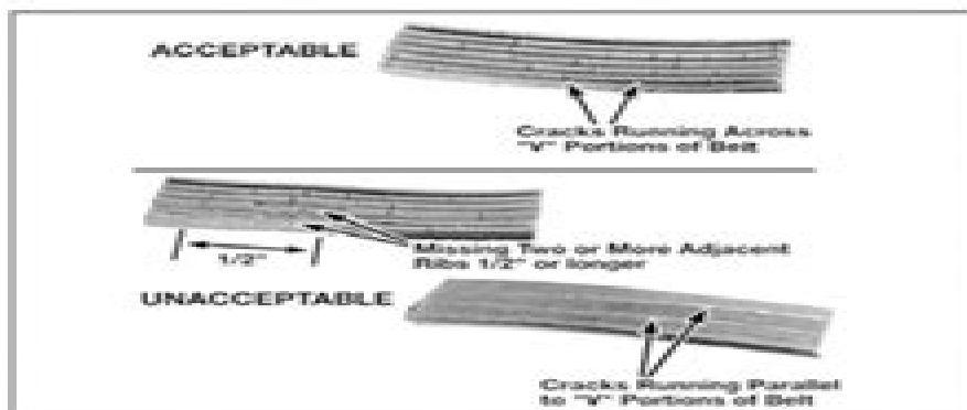
22.4 Small cracks in the underside of a V-ribbed belt are acceptable - lengthwise cracks, or missing pieces that cause the belt to make noise, are cause for replacement
