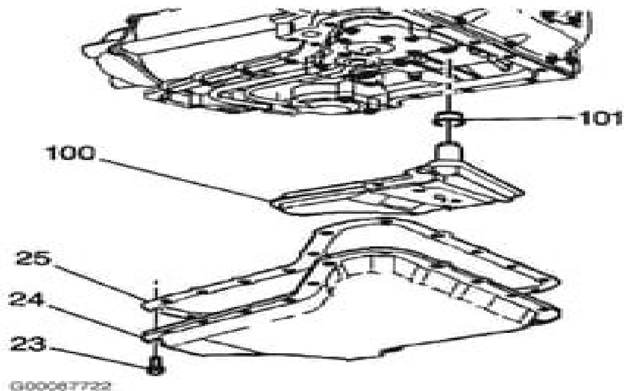
Fig. 3: Removing & Installing Oil Pan & Filter Courtesy of GENERAL MOTORS CORP.
