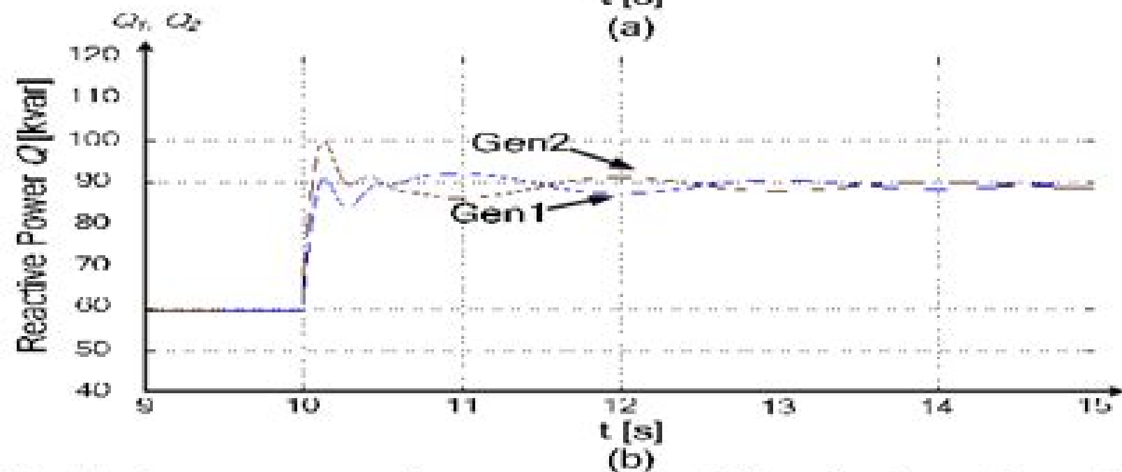
Fig. 13. (a) Generator reactive power using full scale dynamic model and (b) Generator reactive power using dynamic-RMS model.
