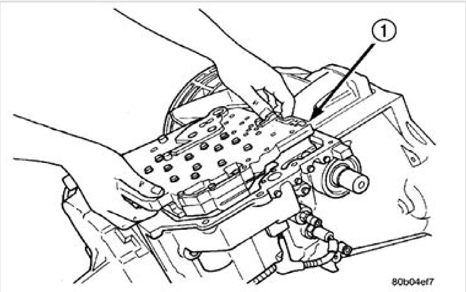
Fig. 412 Valve Body From Transaxle
