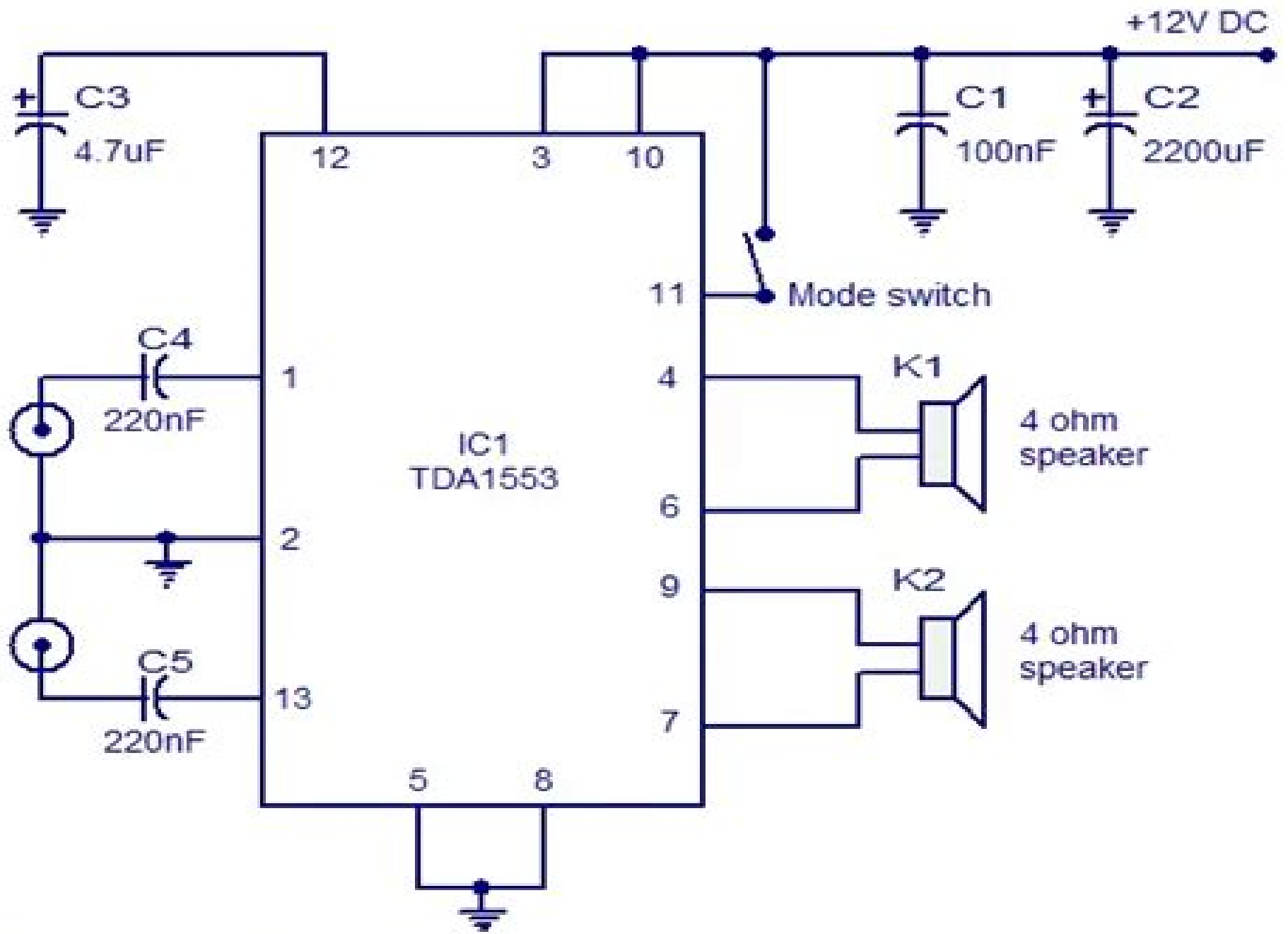
Car stereo amplifier circuit
