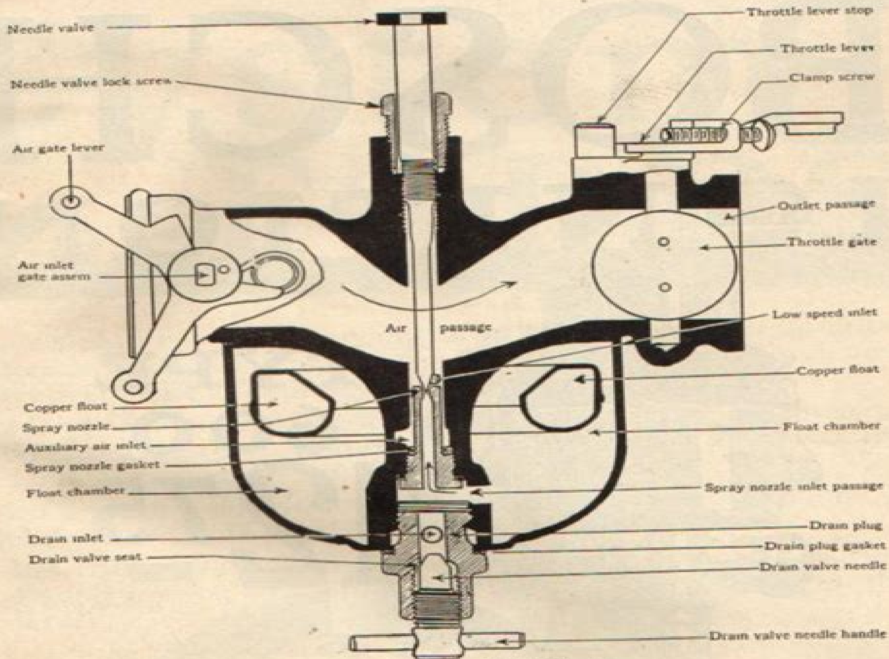
Side Section Holley N H Carburetor
