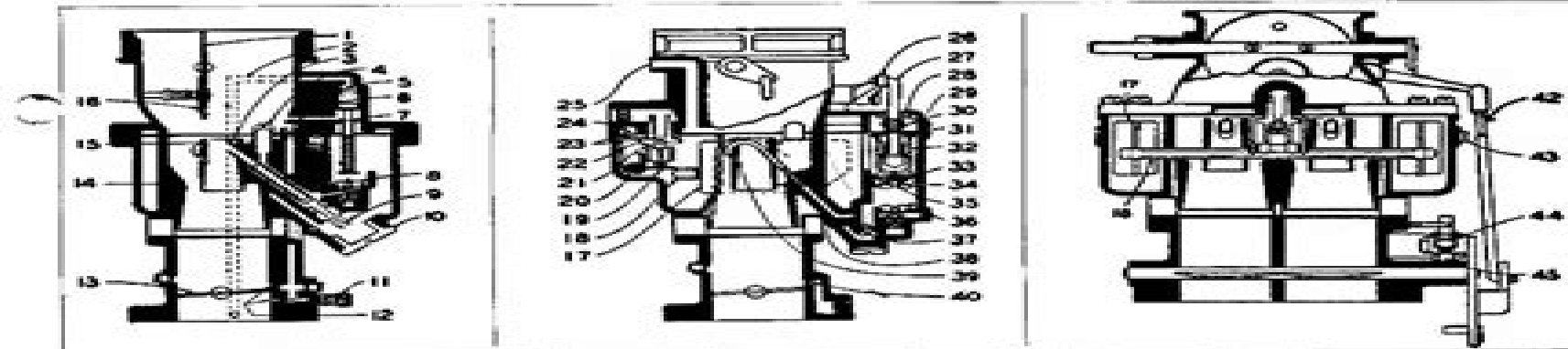
Fig. 1 Three views of Stromberg AAV-2 carburetor. Left: Main metering and vacuum-controlled power system. Center: Acceleration system. Right: Fuel inlet and float system.
