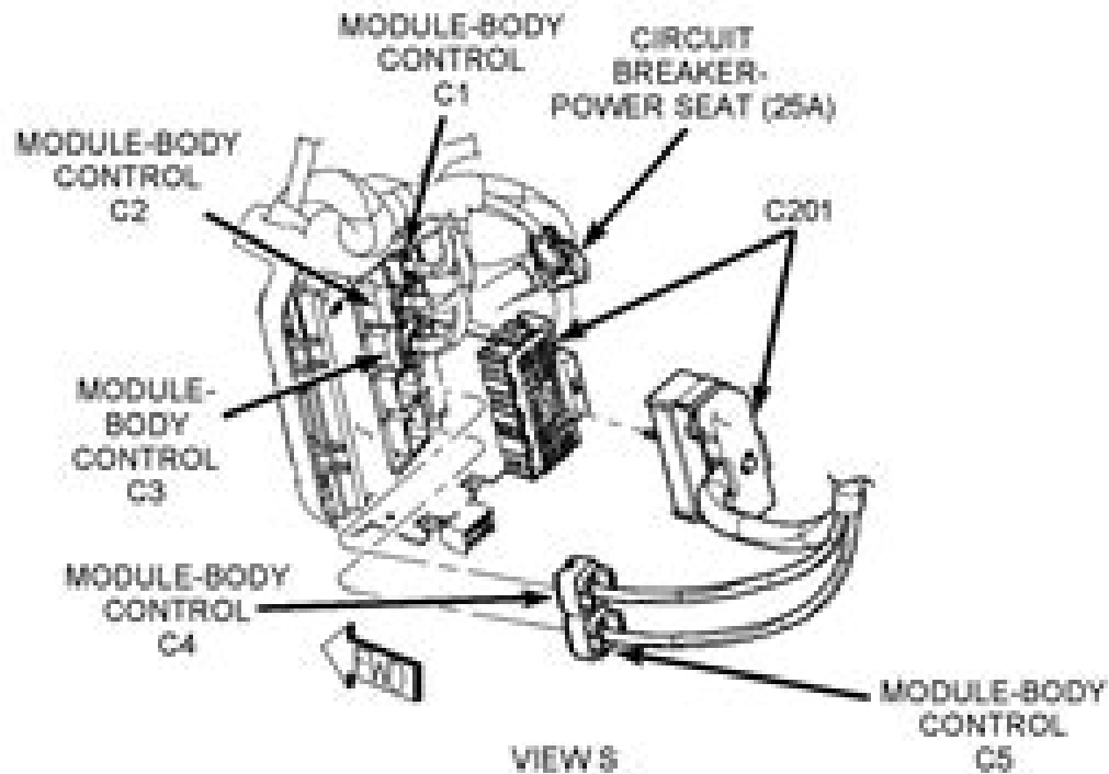
INSTRUMENT PANEL - SIDES
