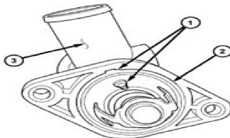
Fig. 21 Thermostat Indexing - 2.0L/2.4L
