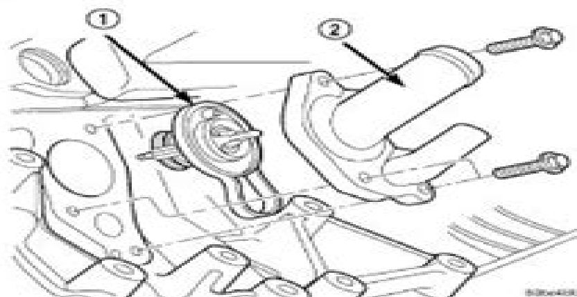
Fig. 20 Thermostat and Housing—2.7L Engine
