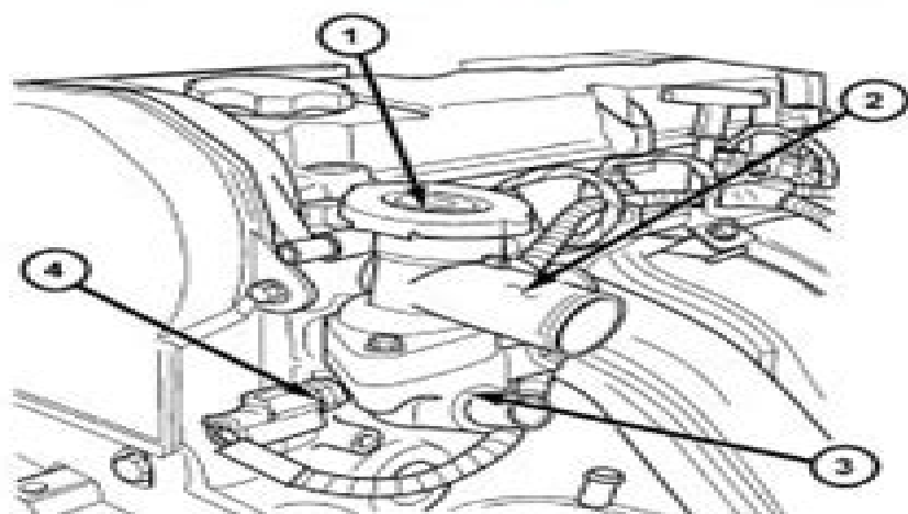
Fig. 19 Coolant Outlet Connector - 2.0L/2.4L
