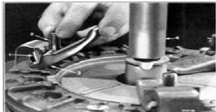
Fig. 63—Assembling Release Lever
