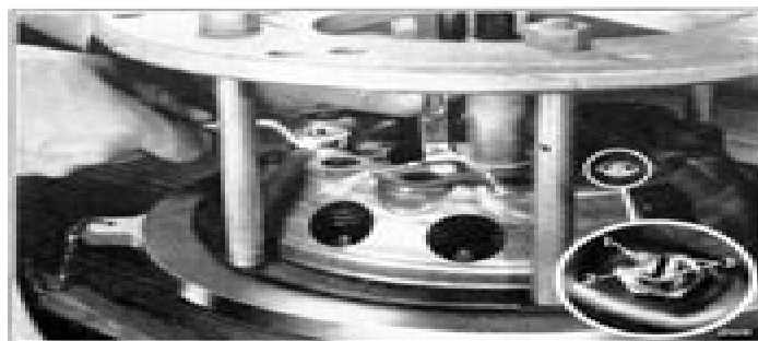
Fig. 65—Adjusting Clutch Release Lever
