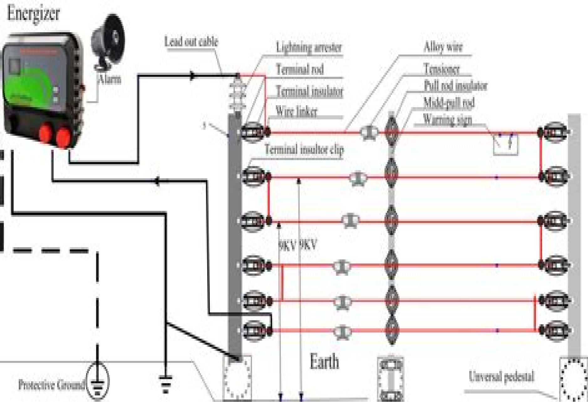
6 Wiring for reference
