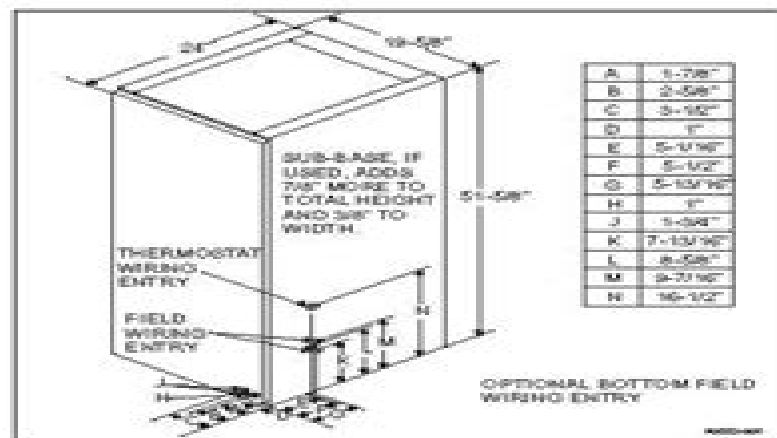
FIGURE 1: Furnace Dimensions
