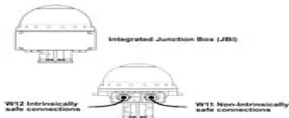
Figure 1. Electrical connections on the TankRadar REX.
