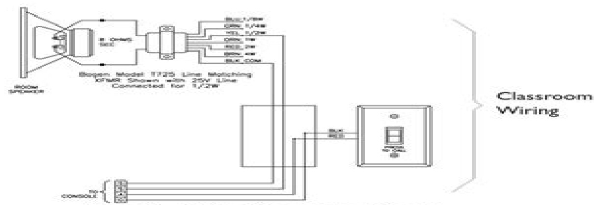
Figure 1 - CA15C Connecting Diagram
