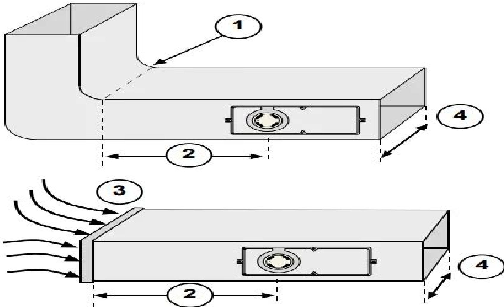
Figure 4: Typical Duct Detector Placement
