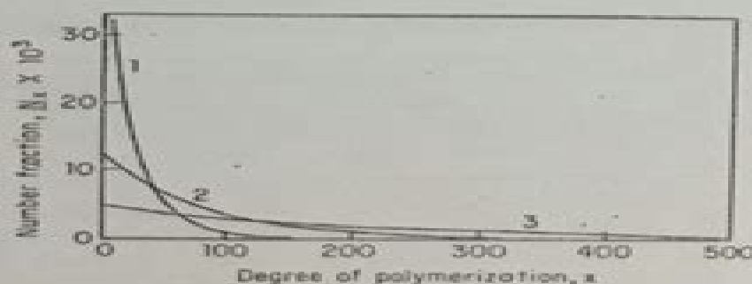
Fig. 2-11 Number fraction distribution curve for linear polymerization. Curve 1: p = 0.9600 ; curve 2: p = 0.9875 ; curve 3: p = 0.9950 . After [52] (by permission of Interscience, Ltd., London).
