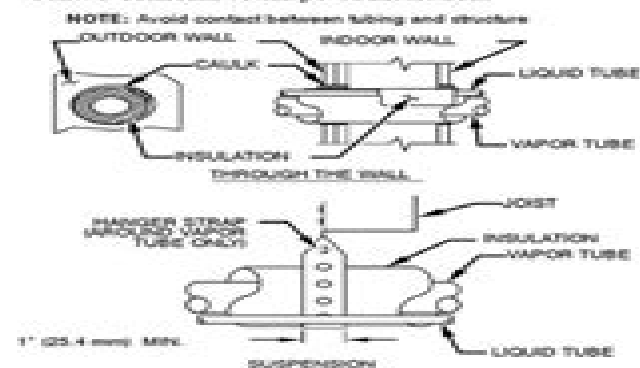
Fig. 1 - Piping Installation
