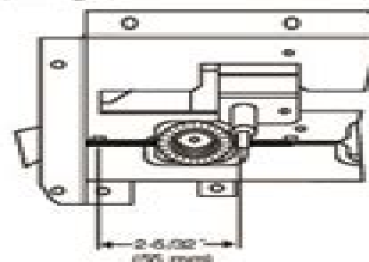
Fig. 14 - Burner Flame
