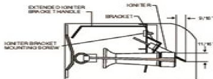
Fig. 13 - Igniter Bracket
