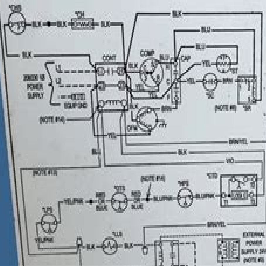
CONNECTION DIAGRAM
