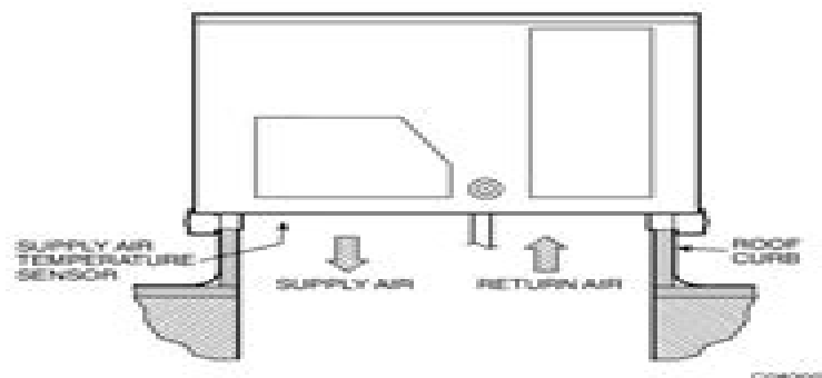
Fig. 42 - Typical Mounting Location for Supply Air Temperature (SAT) Sensor on Small Rooftop Units
