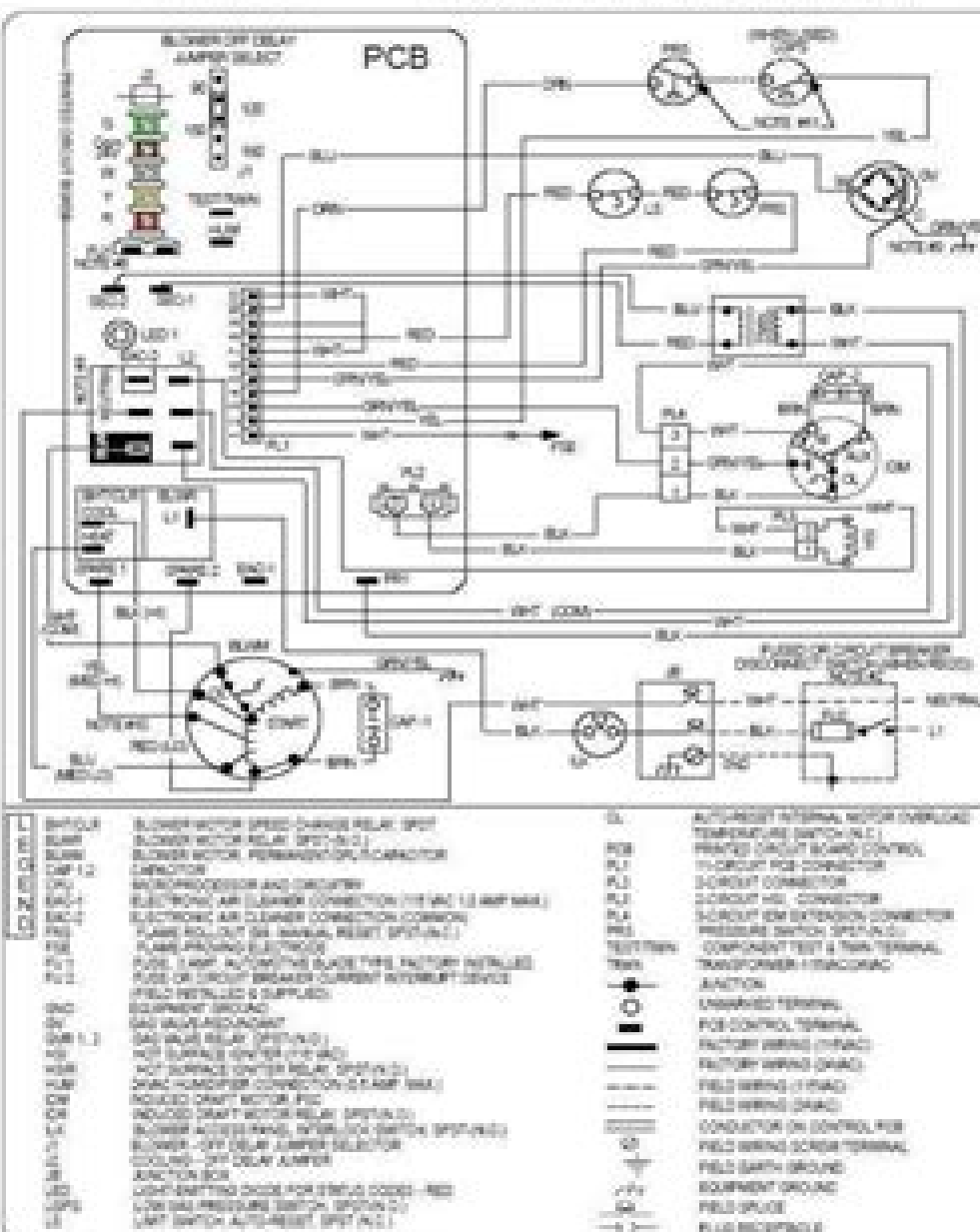
Fig. 18—Wiring Diagram
