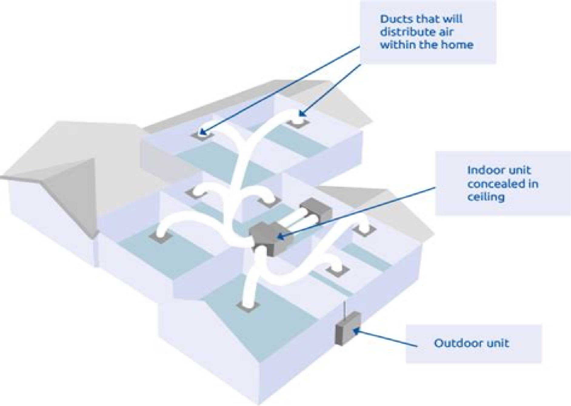
Example of a high static ducted application
