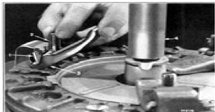
Fig. 63—Assembling Release Lever 1—Strut 2—Eye bolt 3—Release lever 4—Part of tool C-111
