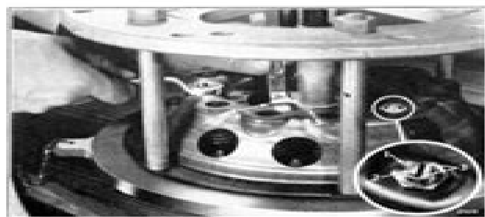
Fig. 65—Adjusting Clutch Release Lever 1—Eye bolt nut 2—Eye bolt 3—Scale bar to lock 4—Adjusting finger, part of tool C-411 5—Spacer, tool C-411-34-A
