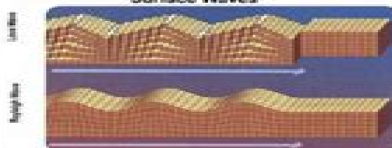
Surface Waves
