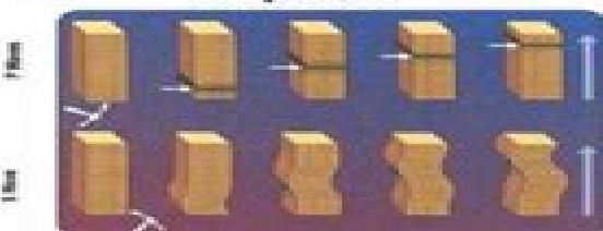
Body Waves
