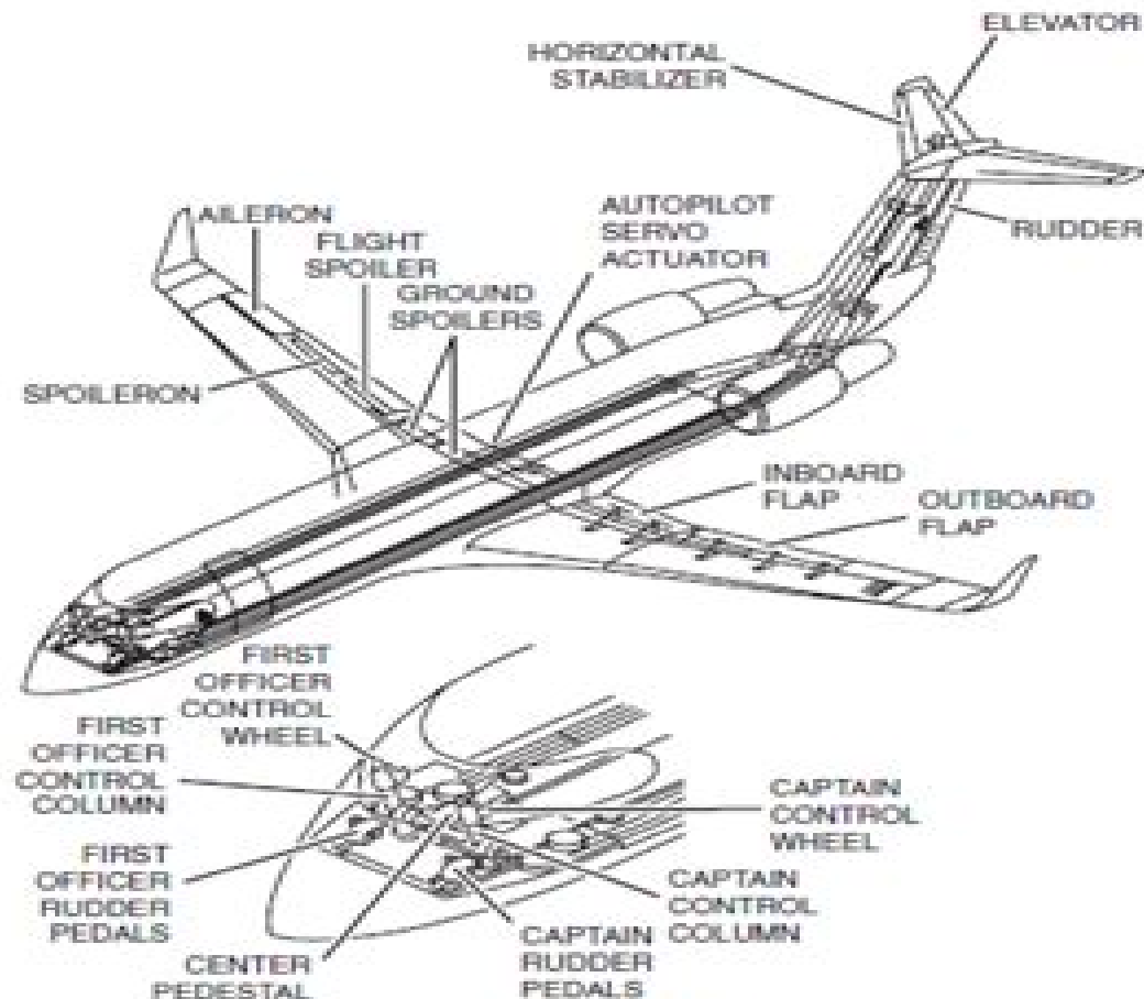
Figure 1-46 Flight Controls
