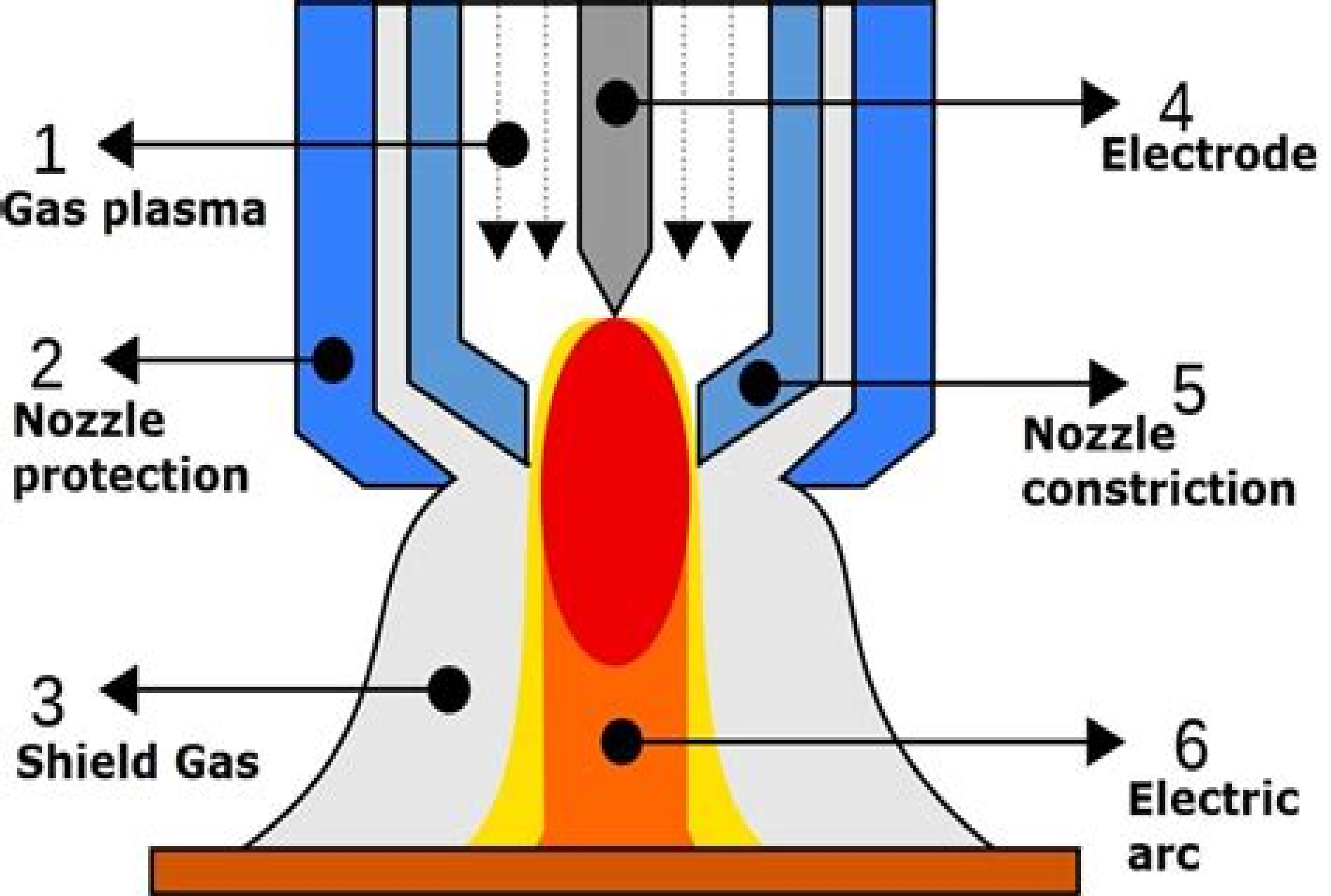
PLASMA ARC WELDING
