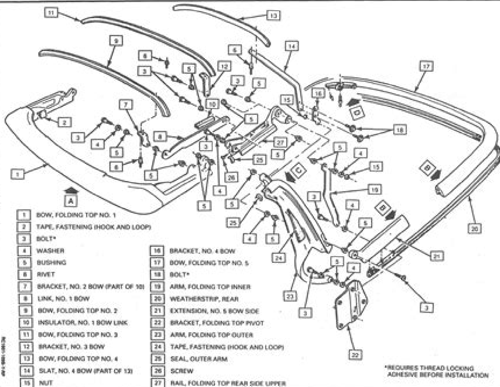
Figure 11 - Top Stack Assembly
