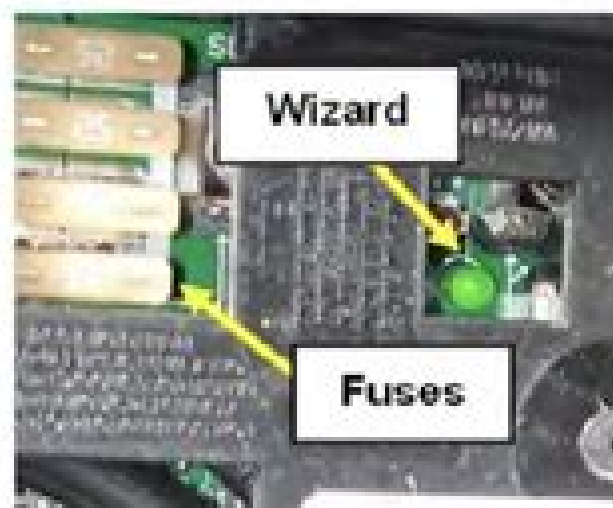
Wizard Button & Reverse Protection Fuses
