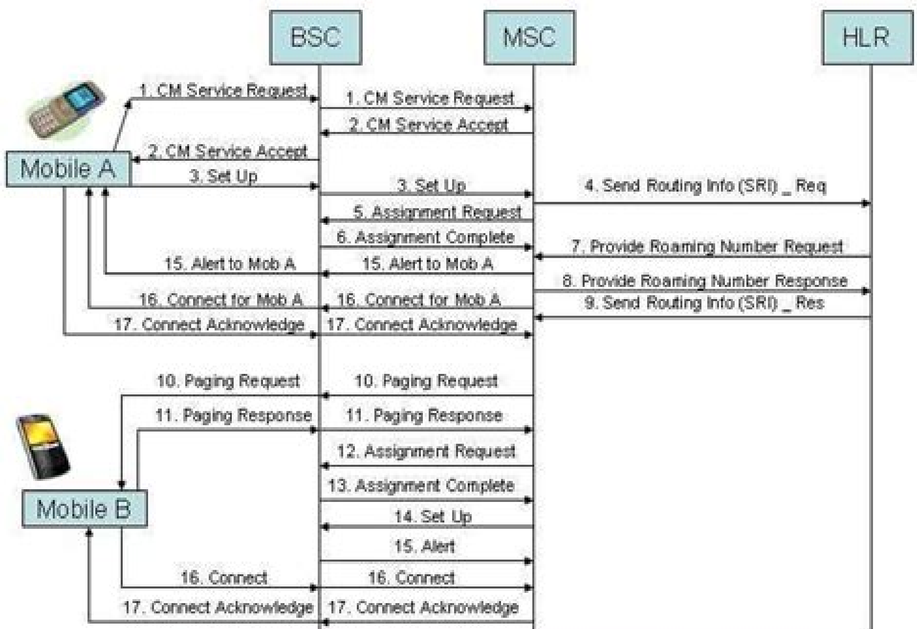
Mobile to Mobile Call Flow, Within Same MSC/BSC
