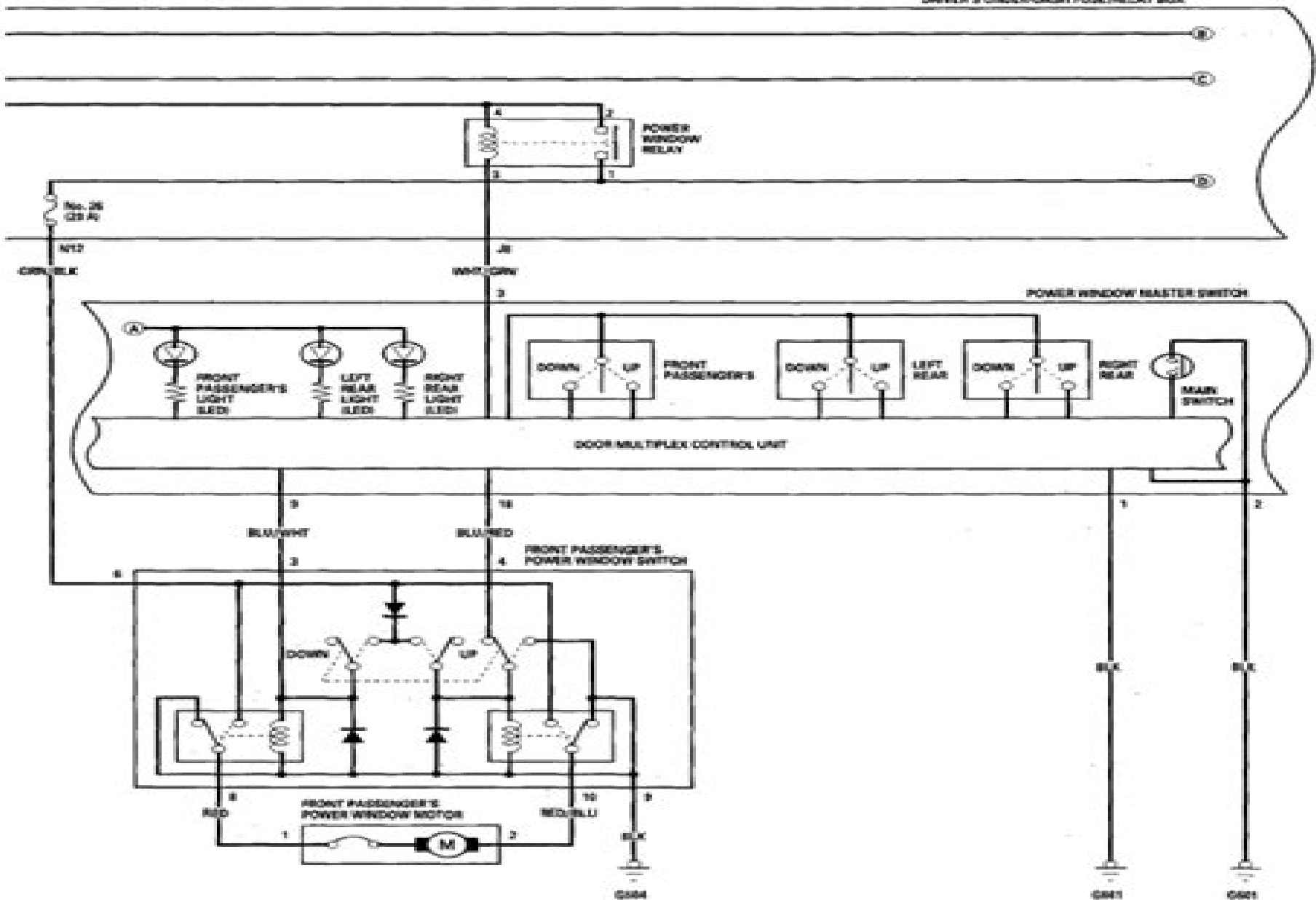
Fig. 5: Power Windows - Circuit Diagram (2 Of 3) Courtesy of AMERICAN HONDA MOTOR CO., INC.
