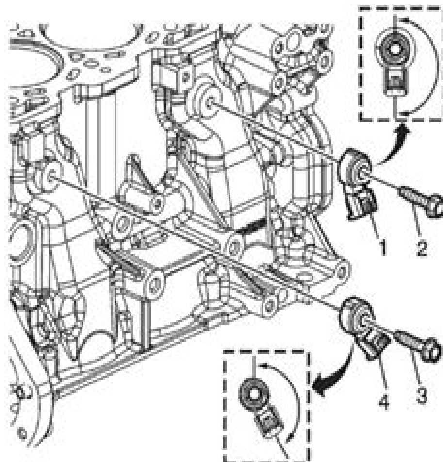
Fig. 213: Knock Sensor
