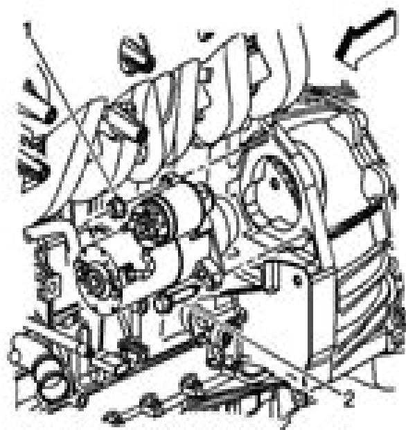
Fig. 30. Reassembly/Installing Starter Motor Courtesy of GENERAL MOTORS CORP.
