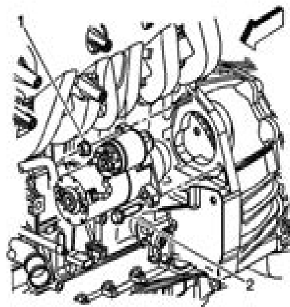
Fig. 31. Reassembly/Installing Starter Motor Courtesy of GENERAL MOTORS CORP.
