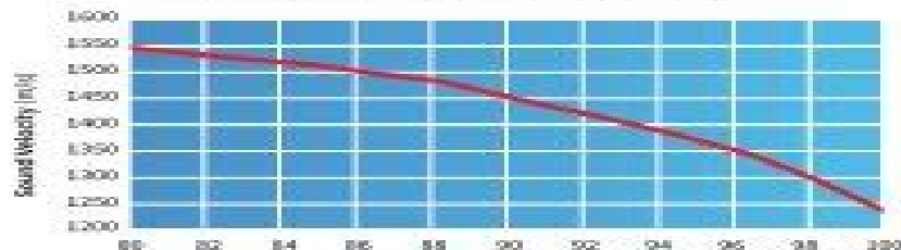
Sulphuric Acid 80..100% wt (25 Deg C)
