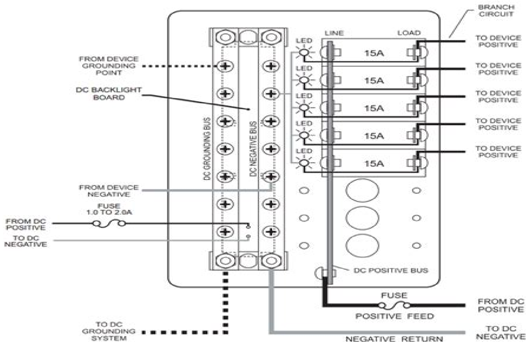
Wiring Diagram DC Power Distribution Panel (PN 8023 /PN 3023 shown for reference)
