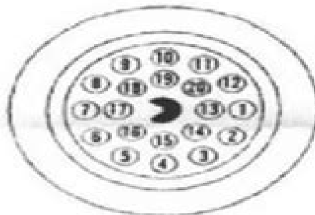
Female Connector (Plug at the car)
