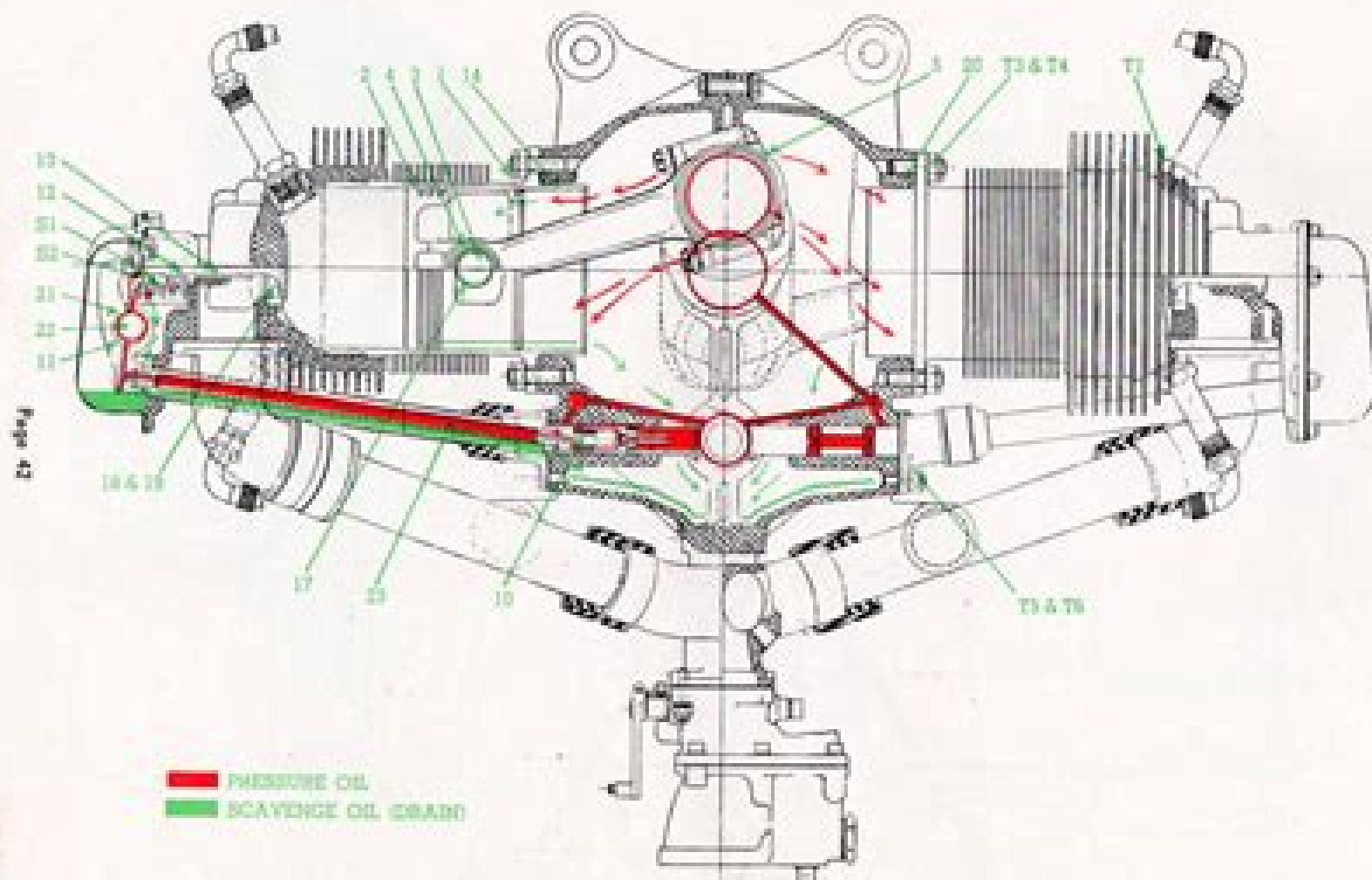
LUBRICATION CHART, CROSS-SECTIONAL VIEW — Figure 27
