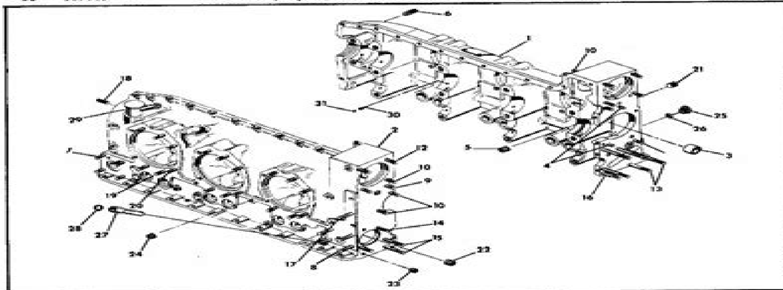
Figure 1. Crankcase Studding Assembly.
