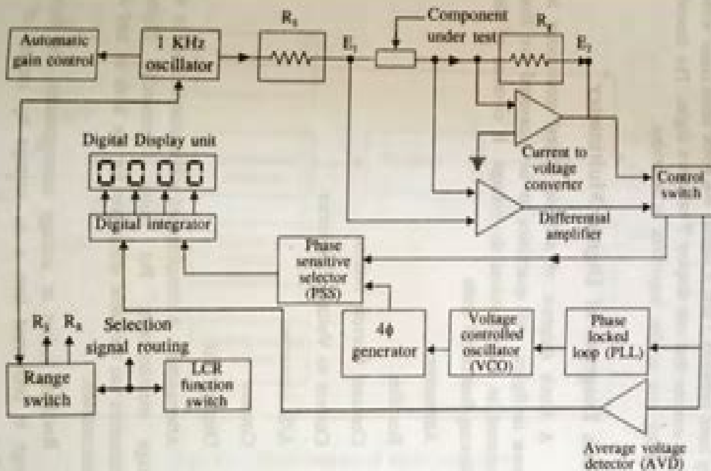
Fig. 9.3 : Block diagram of a digital LCR meter
