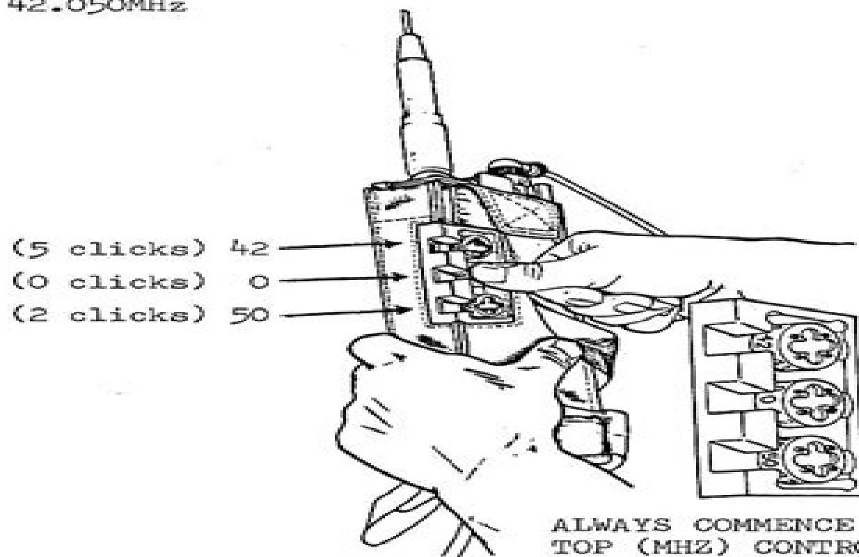
Fig 5 - Frequency Setting
