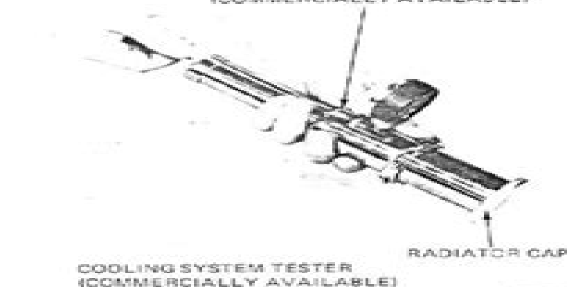
COOLING SYSTEM TESTER (COMMERCIALLY AVAILABLE)
