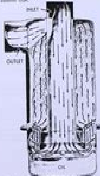
Figure 20 — Section View of Oil Bath Air Cleaner
