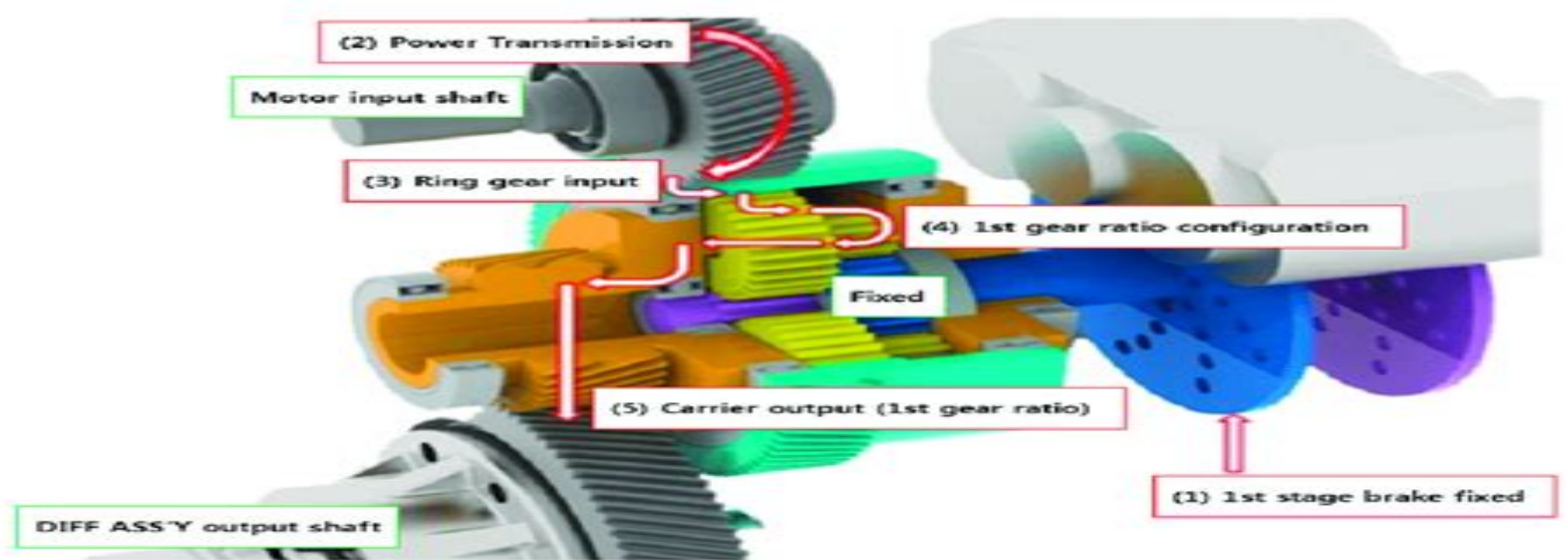
1st gear shift mechanism
