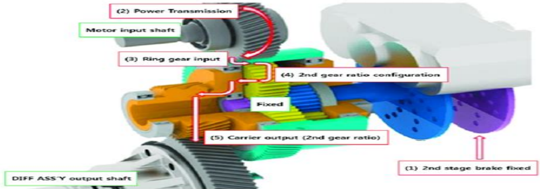
2nd gear shift mechanism
