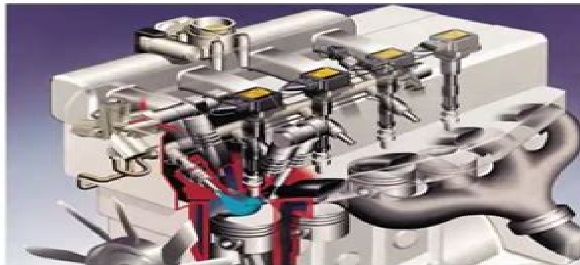
Figure 10.30 Gasoline direct injection on an engine (Source: Bosch Media)
