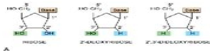
STRUCTURE OF RIBOSE, DEOXYRIBOSE, AND DIDEOXYRIBOSE
