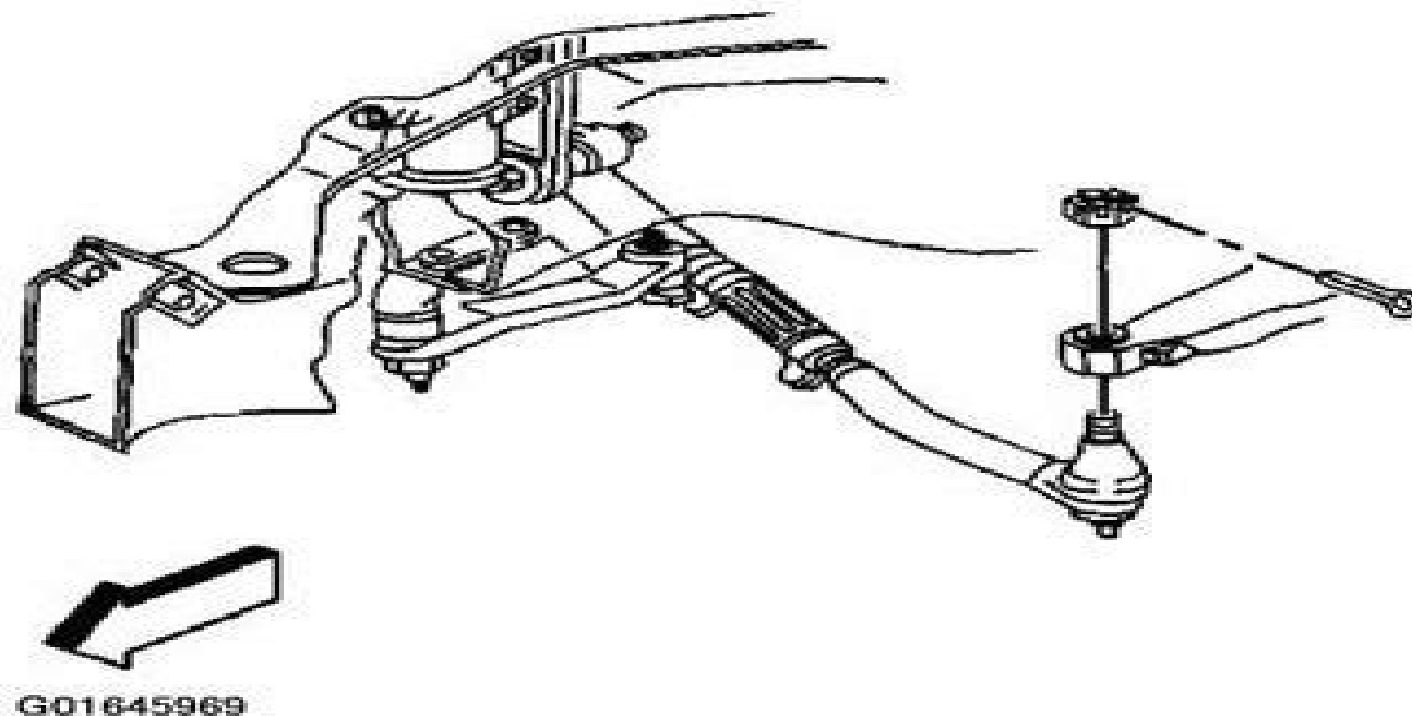
Fig. 2: Removing Cotter Pin And Castellated Nut From Outer Tie Rod Courtesy of GENERAL MOTORS CORP.
