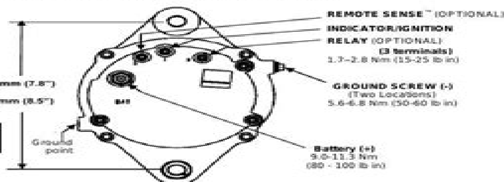
FIGURE 1: 28SI ALTERNATOR TORQUE VALUES
