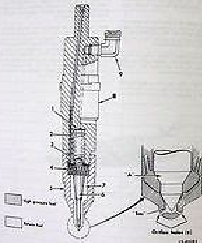
Fig. 1 - Schematic View of Nozzle (Fig. 1) (Fig. 1) (Fig. 1)
